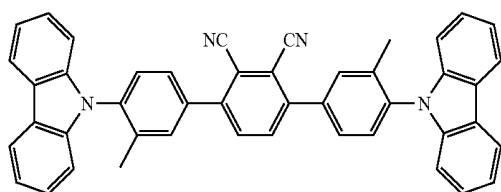
Compound 15
