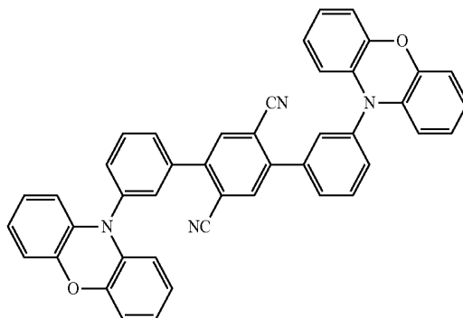
Compound 13
