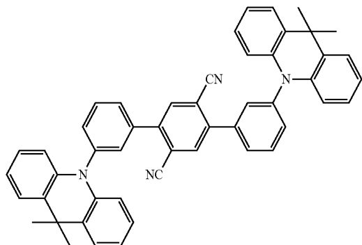
Compound 11
