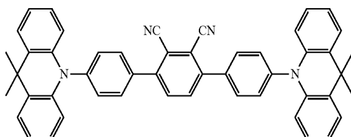
Compound 16
