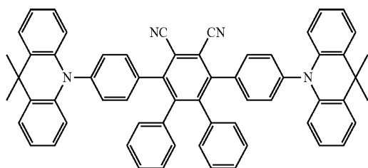
Compound 29
