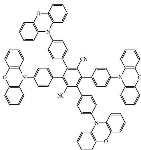
Compound 9
