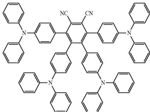
Compound 27
