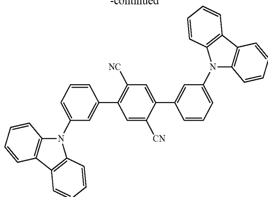
Compound 3
