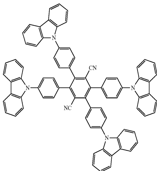
Compound 7
