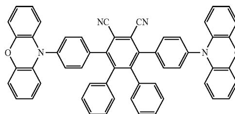
Compound 30
