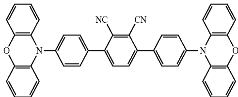
Compound 17
