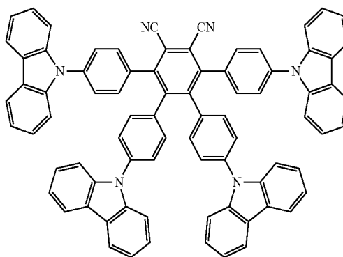
Compound 24
