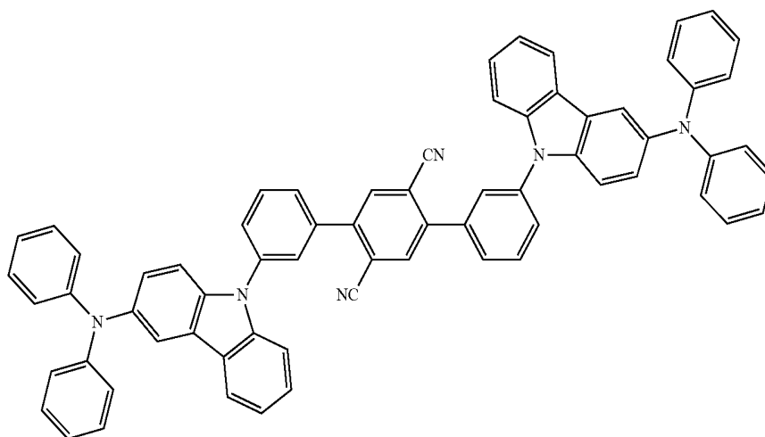
Compound 15
