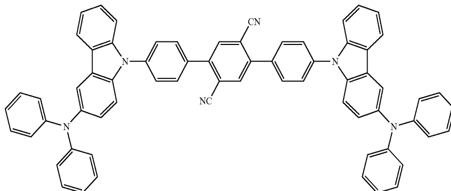
Compound 7
